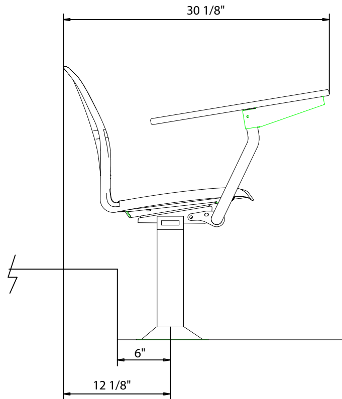
3-CHAIR HORIZONTAL BAR MOUNT
